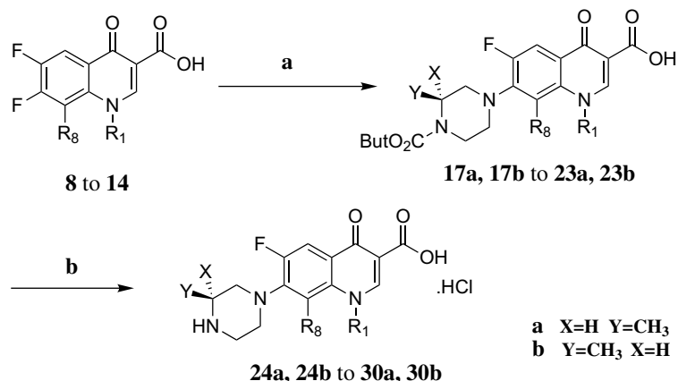
Scheme 3. Reagents and conditions: (a) 3a or 3b , N -methylmorpholine/DMSO; (b) 3 N HCl/EtOH.
